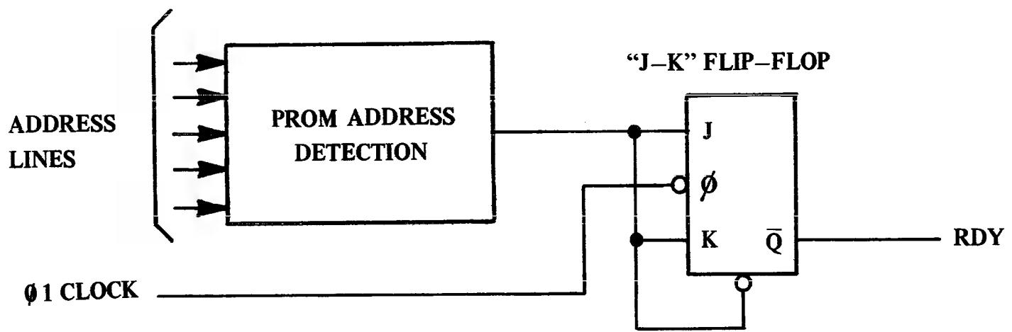
Interfacing Scheme for Slow PROM's FIGURE 2.16
